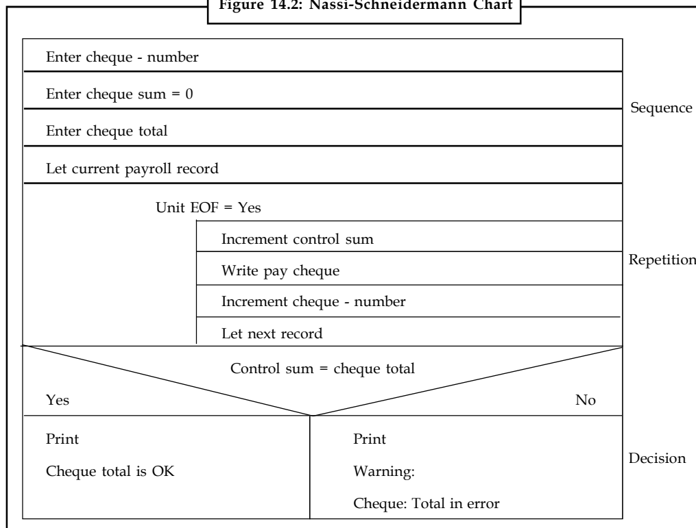
Figure 14.2: Nassi-Schneidermann Chart
